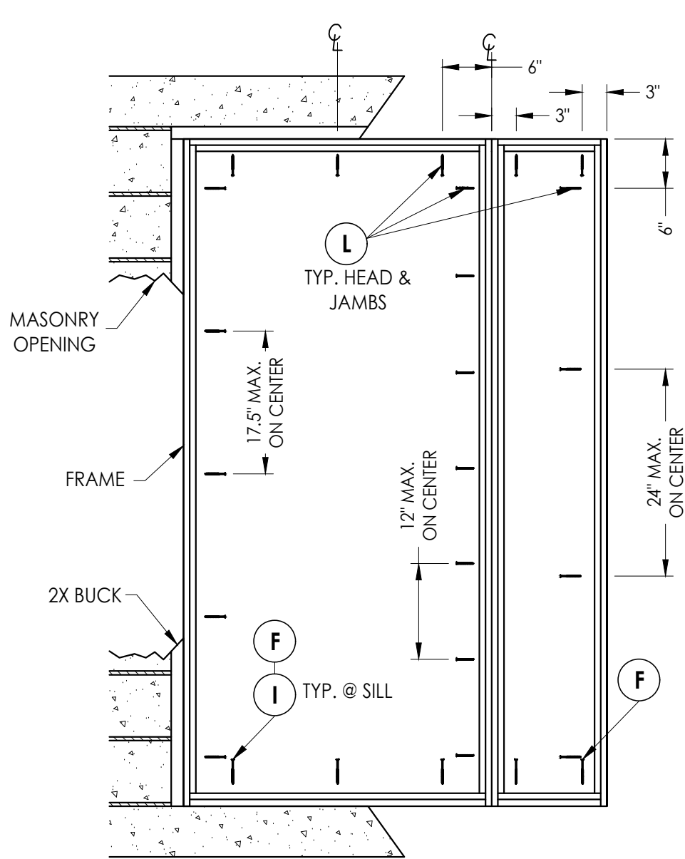
FRAME ANCHORING
