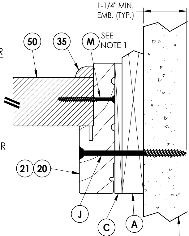
5 HORIZONTAL CROSS SECTION 4 Shown w/1X sub-buck
